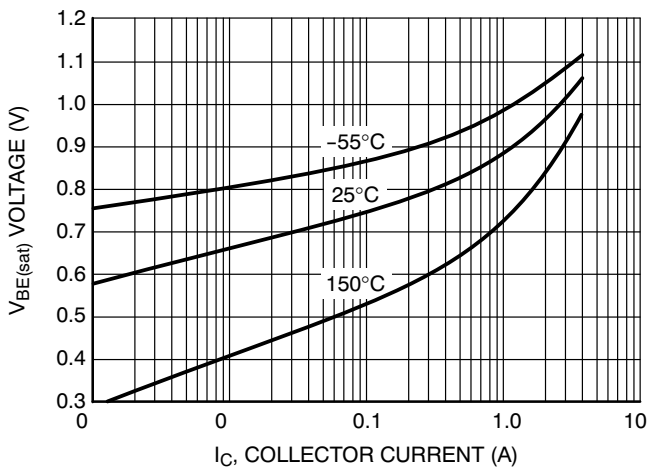
Figure 3. V_{BE(sat)}
