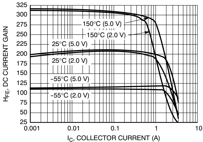
Figure 2. DC Current versus Collector Current
