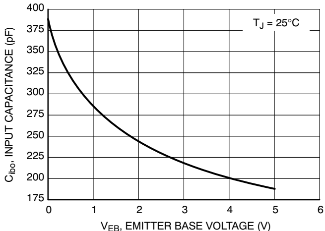
Figure 6. Input Capacitance
